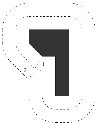
Figure 4: Fattening of a set; exercise 9.70
