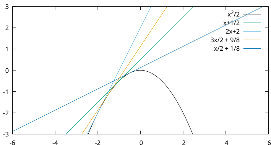
Figure 12: Solution of 22.22: envelope.
