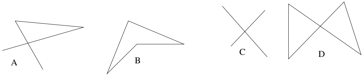
Figure 7: Sets for exercise E20.12
